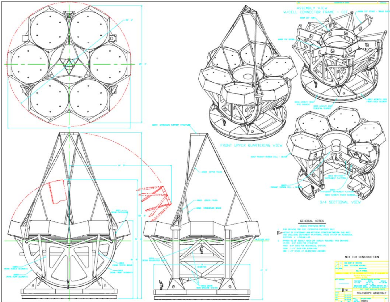
Engineering sketches offer a glimpse of the technical grandeur of the Grand Magellan. 1) Top left: The seven-segment design was chosen to take advantage of the current state of technology in casting large mirrors. Six segments are "off axis," or offset from the center segment. The center segment is "on axis." 2) Bottom left: The telescope is considered an "alt az" design: The entire structure rides on a circular track for azimuth positioning, and the upper structure is elevated with giant C-rings for altitude control. The moving mass of the telescope is 1,100 tons. 3) Top right: Light reflects from the seven primary mirrors up to seven secondary mirrors 115 feet above the floor. They are supported by carbon-reinforced steel legs. 4) Bottom right: Light reflected from the secondary mirror passes through a hole in the central primary mirror and is received by scientific instruments located on a platform underneath. Instruments are raised and lowered via an elevator in the core of the telescope pier structure. DRAWINGS COURTESY OF PARAGON ENGINEERING/CARNEGIE OBSERVATORIES.
